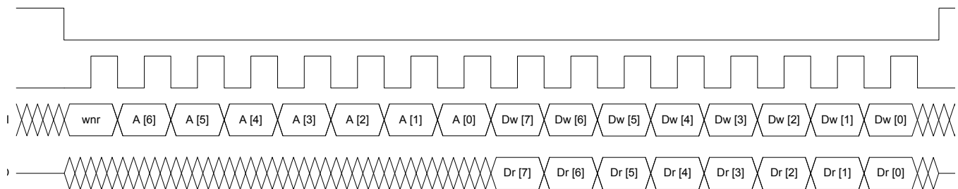
Figure 4-1: SPI Timing Diagram (Single Access)
