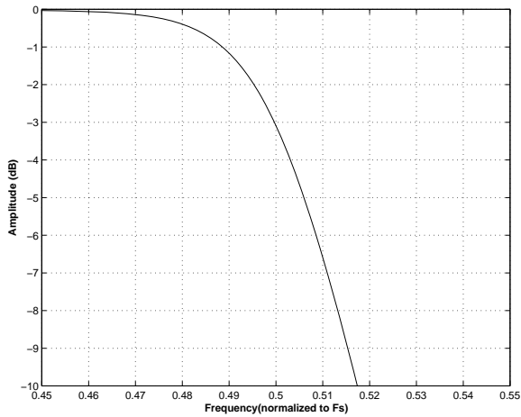
Figure 34. Single-Speed (slow) Transition Band (detail)
